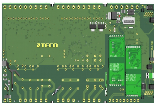
Fig.7.1 Placement of replaceable submodules with serial channel interface on the bottom plate of the CP-2000 base module
