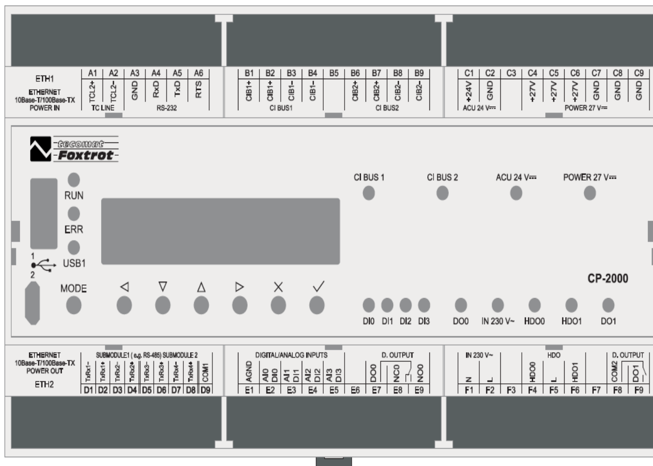
Fig. 4.1 Connection of binary and analog inputs/outputs of basic module CP-2000
